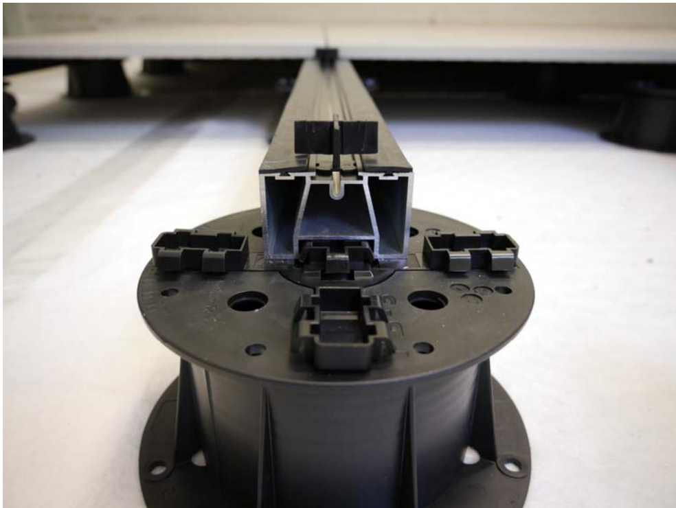
Figure B.2. Pedestal Buzon PB-3 with Kit 2 and support profile.
