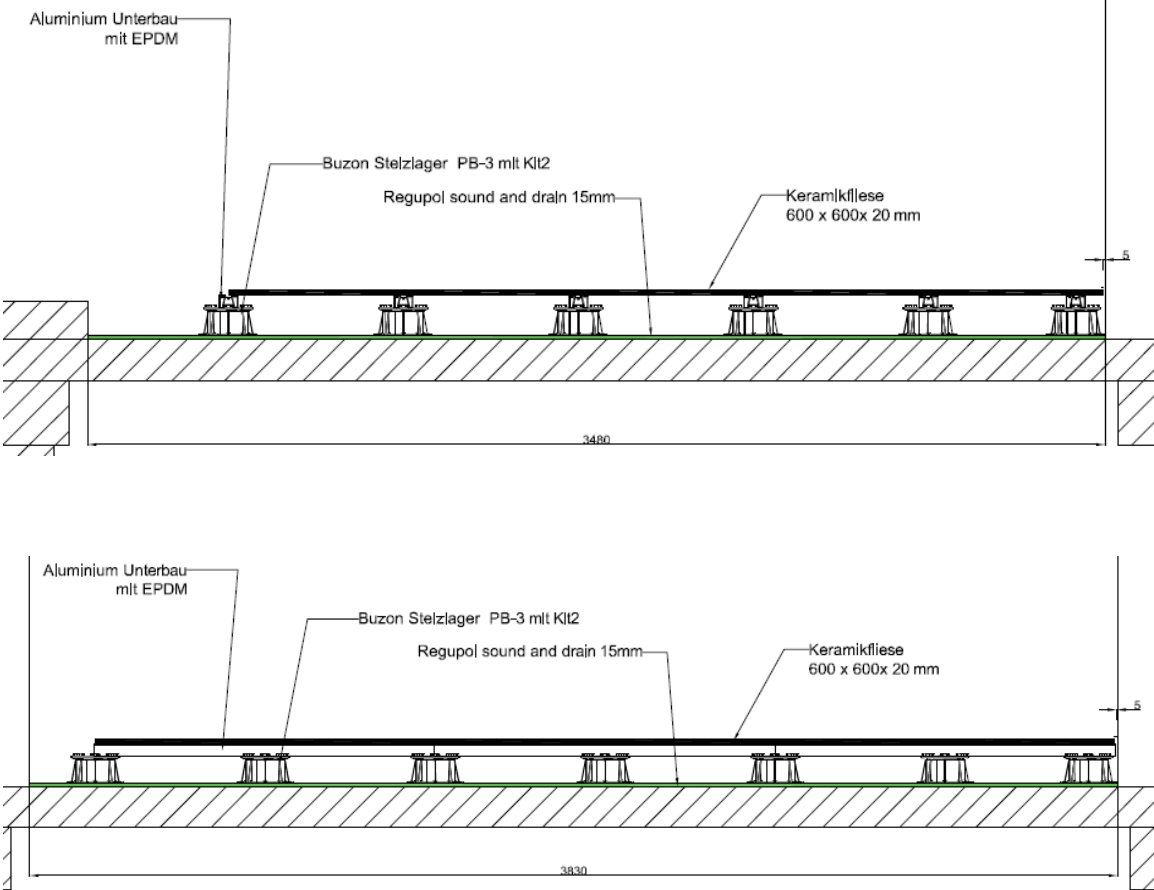
Figure C.3. Test setup in the ceiling test facility: structure details, cross section and longitudinal section.
