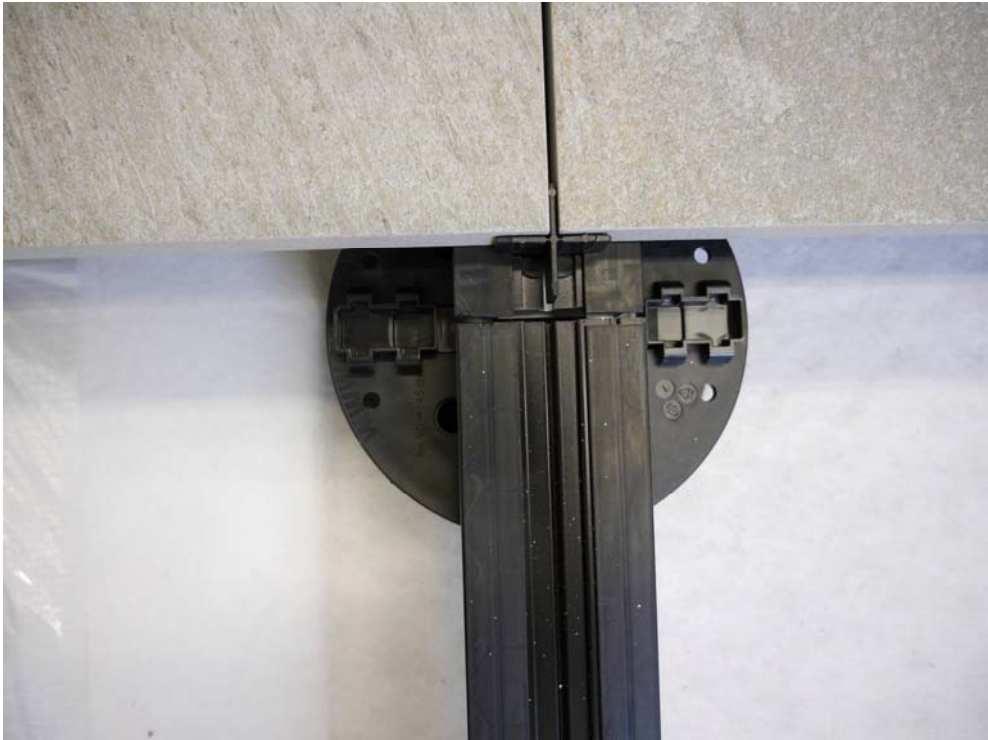
Figure B.4. Test setup during mounting: pedestals with support profiles and partly laid ceramic tiles.
