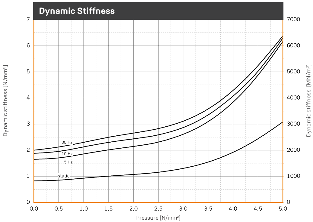
Illustration of the dynamic stiffness for sinusoidal excitation at a constant mean load and an amplitude of ± 0.10 mm. Dimensions of specimens 125 x 125 x 25 mm; static stiffness as a result of the tangent modulus of the spring characteristic. Tested in accordance with DIN 53513.
