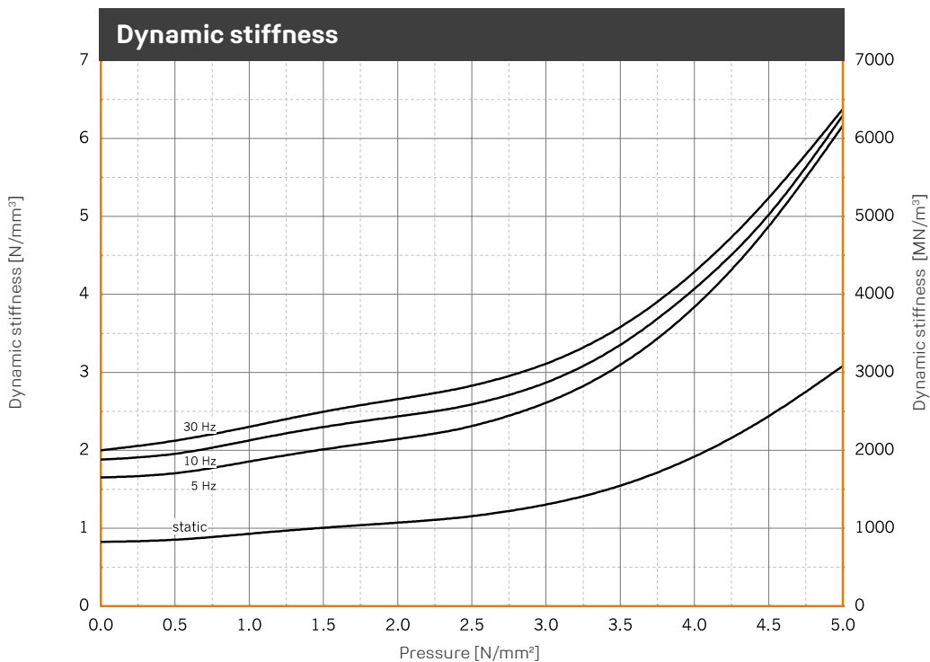
Illustration of the dynamic stiffness for sinusoidal excitation at a constant mean load and an amplitude of \pm 0.10 mm. Dimensions of specimens 125 x 125 x 25 mm; static stiffness as a result of the tangent modulus of the spring characteristic. Tested in accordance with DIN 53513.
