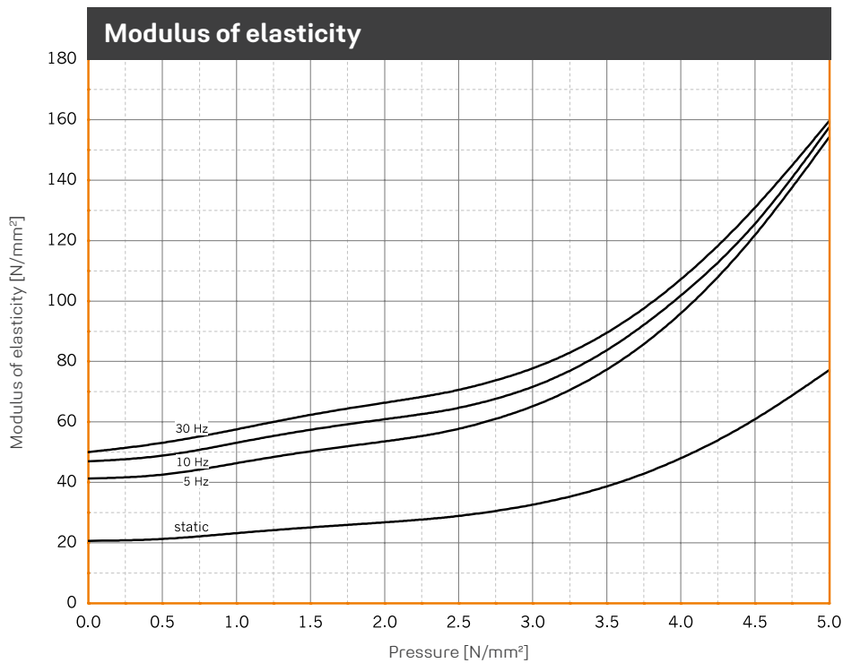
Illustration of the dynamic modulus of elasticity for sinusoidal excitation at a constant mean load and an amplitude of \pm 0.10 mm. Dimensions of specimens 125 x 125 x 25 mm; static modulus of elasticity as a result of the tangent modulus of the spring characteristic. Tested in accordance with DIN 53513.
