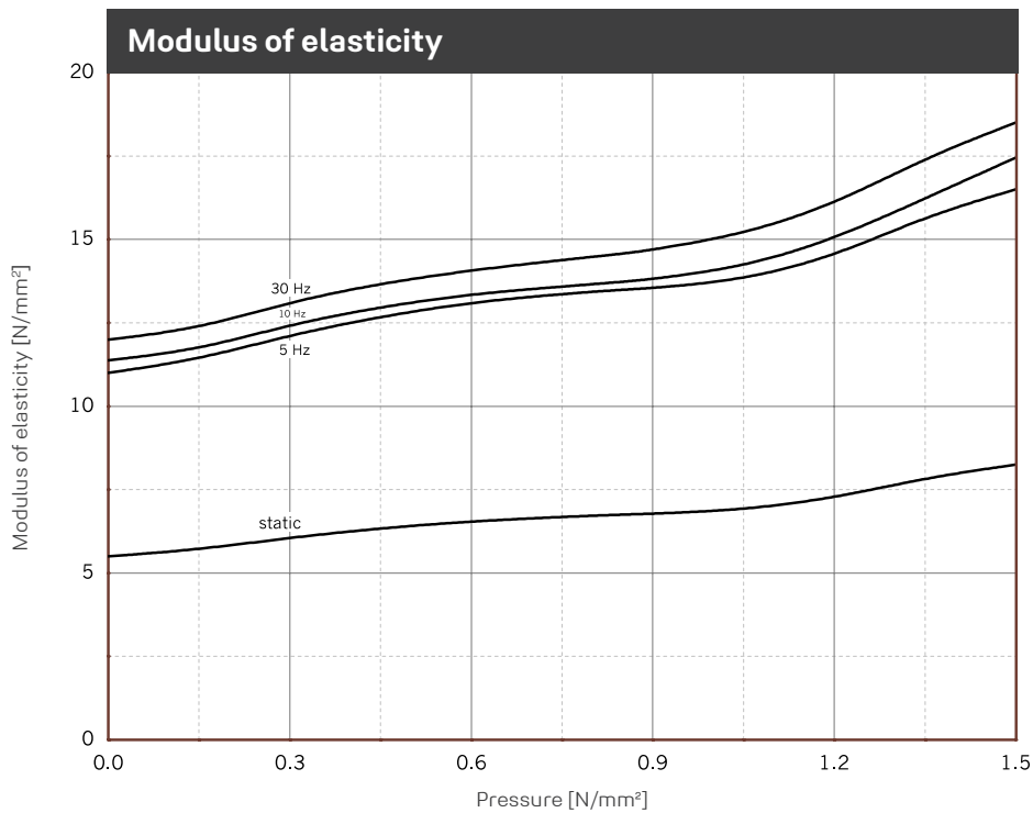
Illustration of the dynamic modulus of elasticity for sinusoidal excitation at a constant mean load and an amplitude of ± 0.10 mm. Dimensions of specimens 250 x 250 x 25 mm; static modulus of elasticity as a result of the tangent modulus of the spring characteristic. Tested in accordance with DIN 53513.
