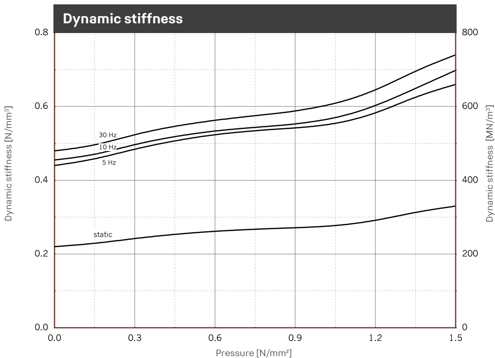
Illustration of the dynamic stiffness for sinusoidal excitation at a constant mean load and an amplitude of ± 0.10 mm. Dimensions of specimens 250 x 250 x 25 mm; static stiffness as a result of the tangent modulus of the spring characteristic. Tested in accordance with DIN 53513.
